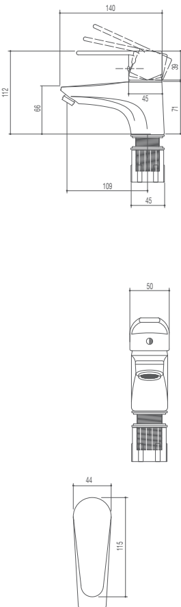
Single lever single-hole basin mixing faucet
