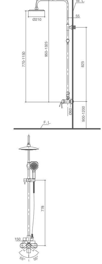
Square lever handle, 6" wall mounted bath mixing faucet, 8" sunflower head and hand shower with adjustable holder on brass pipe
