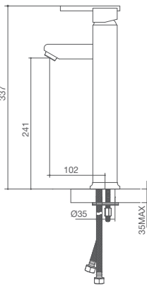
Square lever handle single hole elongated basin mixing faucet
